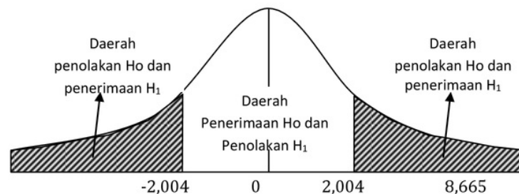
Gambar 3 Kurva Pengujian Independent Sample T-Test
