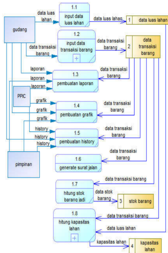
Figure 4 DFD Level 1
