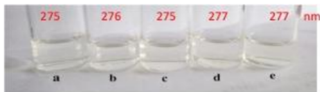
Fig. 3. Photos of NBP after UV exposure for different times (h): 1 (a), 2 (b), 3 (c), 6 (d) and 12 (e). The UV absorbance maximum of each sample is shown in the upper series
