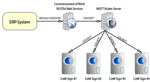
Fig. 1. Block Diagram of Commencement of Work Sign
