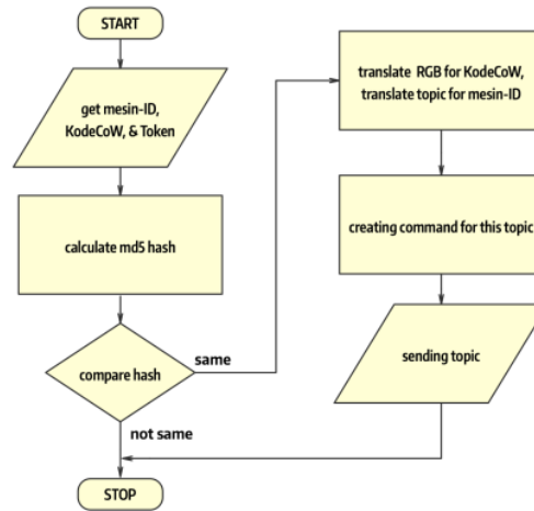
Fig. 3. RESTful API Flowchart
