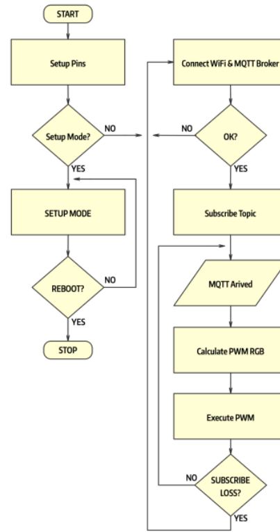
Fig. 4. CoW Sign Flowchart
