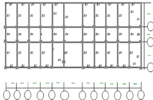
Fig 1: The Floor Beam System
