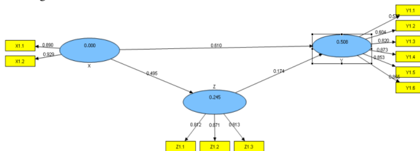
Gambar 2 Diagram PLS
