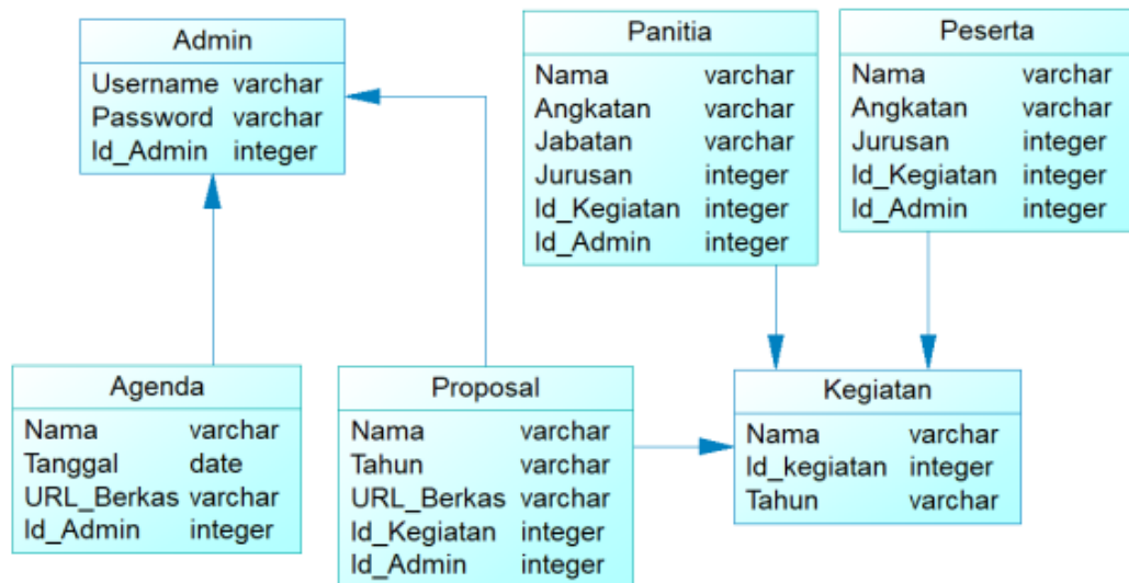
Gambar 3.9 Physical Data Model (PDM)
