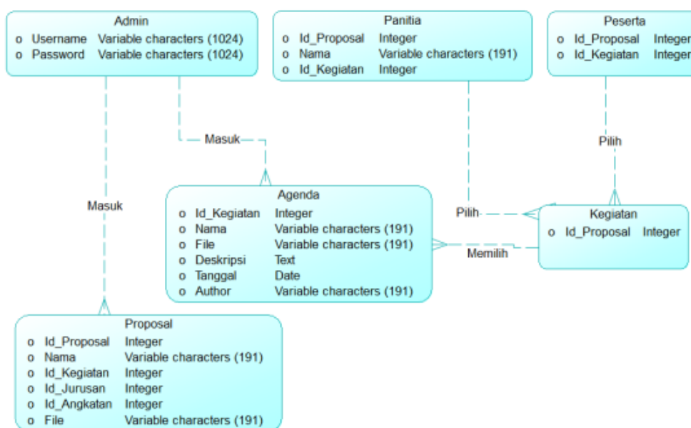
Gambar 3.8 Conceptual Data Model (CDM)
