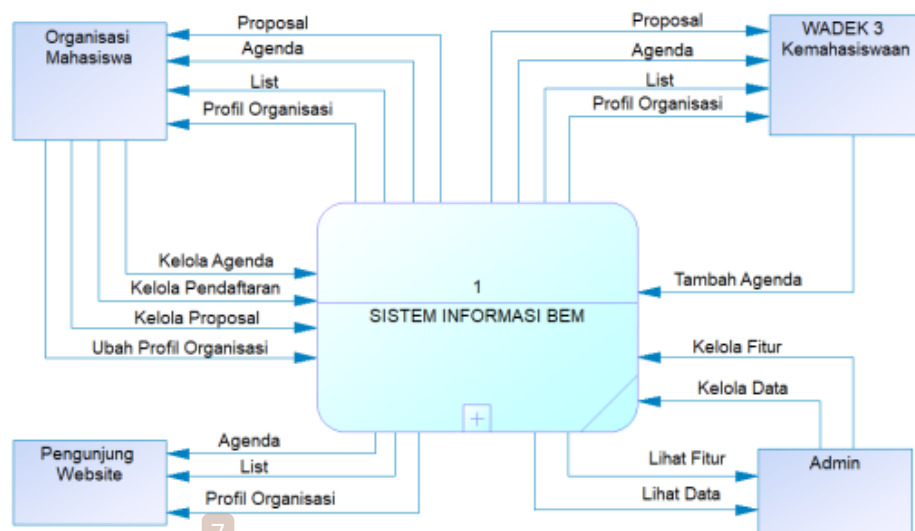
Gambar 3.2 DFD Level Context
