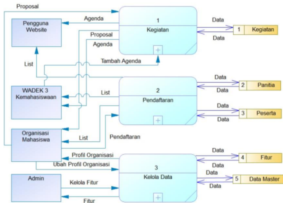
Gambar 3.3 DFD Level 1
