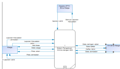
Gambar 4. DFD Context Diagram
