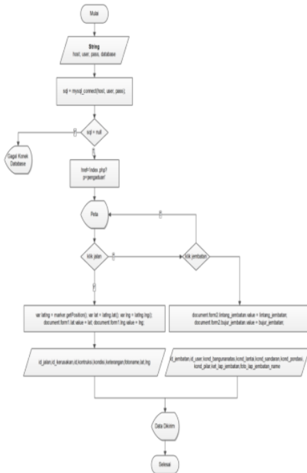
Gambar 10. Flowchart Pengaduan
