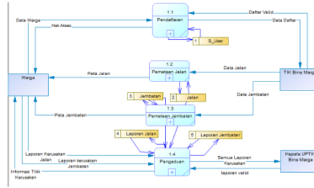
Gambar 5. DFD Level 1
