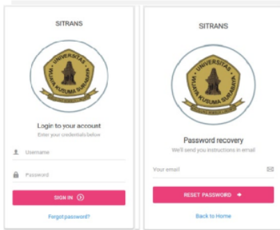
Figure 9 Login Page
