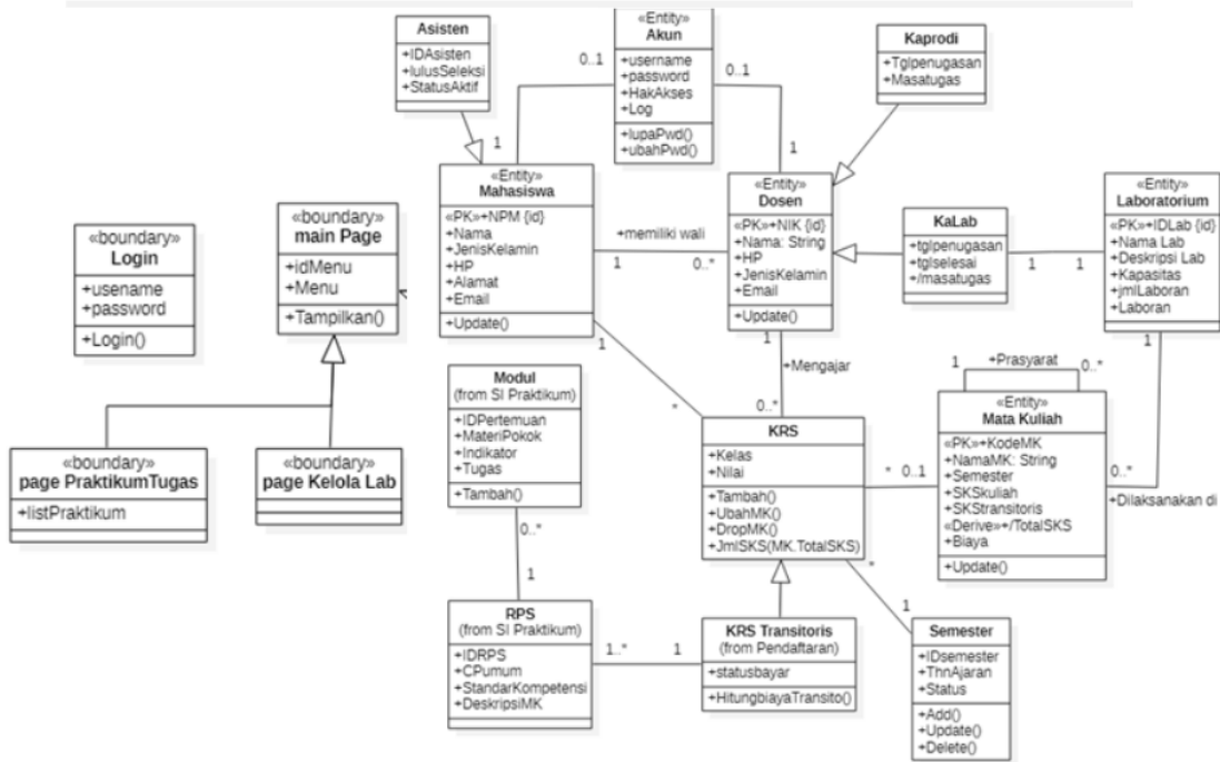
Figure 4 Class Diagram of SITRANS
