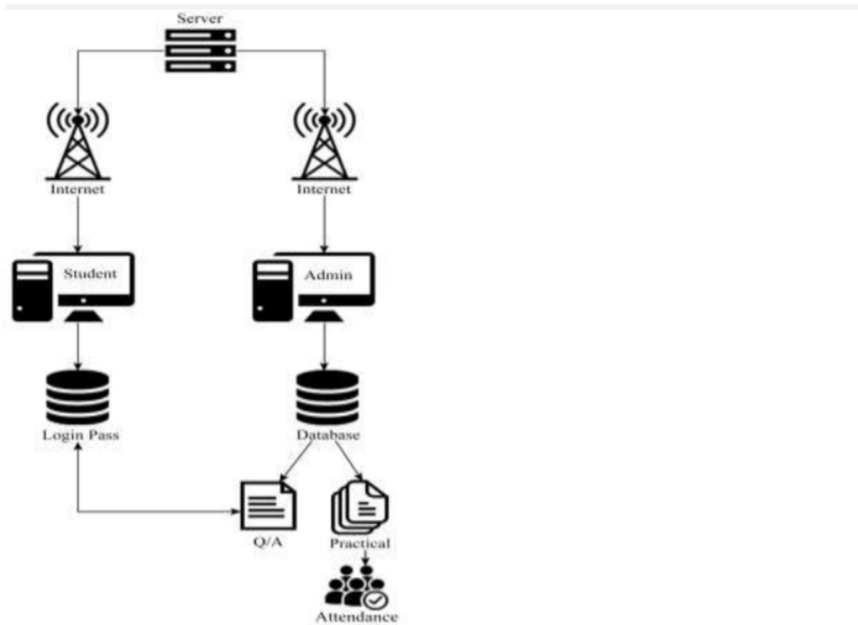
Figure 1 Lab Management System Architecture (Utekar, et al., 2020)
