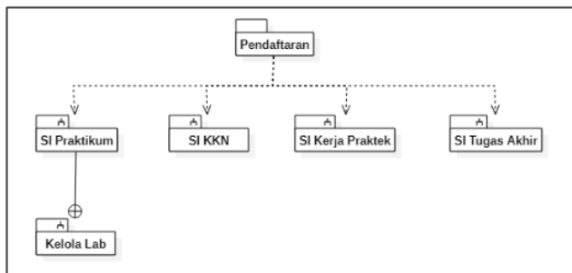
Figure 2 Package Diagram of SITRANS
