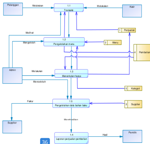
Gambar 6. DFD Level 1
