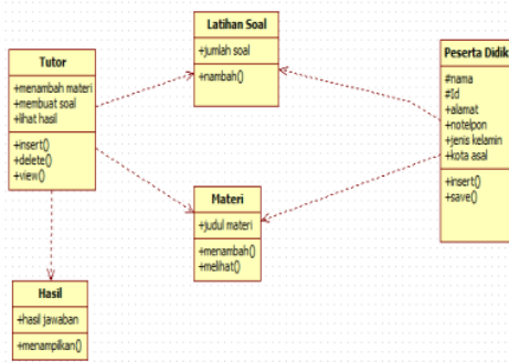
Gambar 5. Class Diagram
