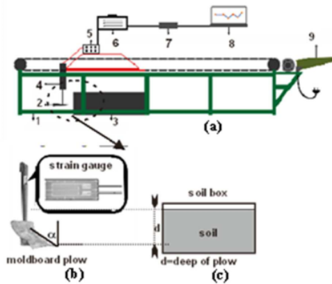
Fig. 1. Part of soil bin tools [18]
