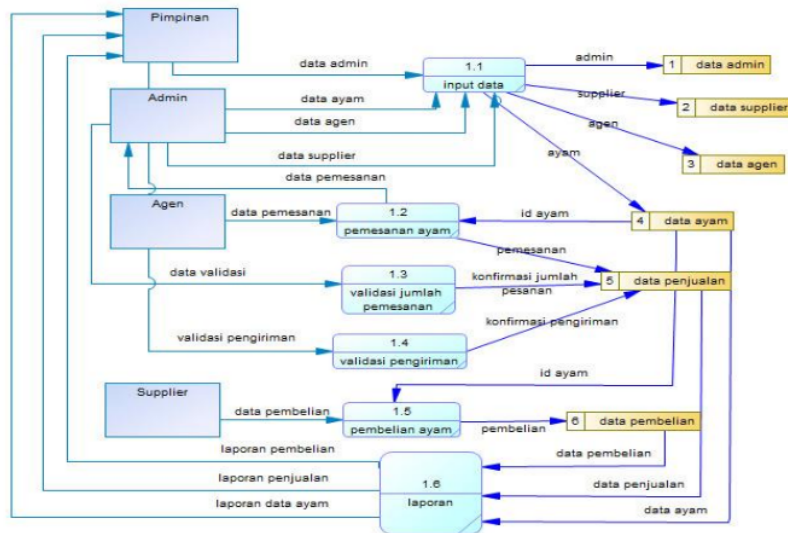
18 Gambar 3.2 Proses DVD Level 1
