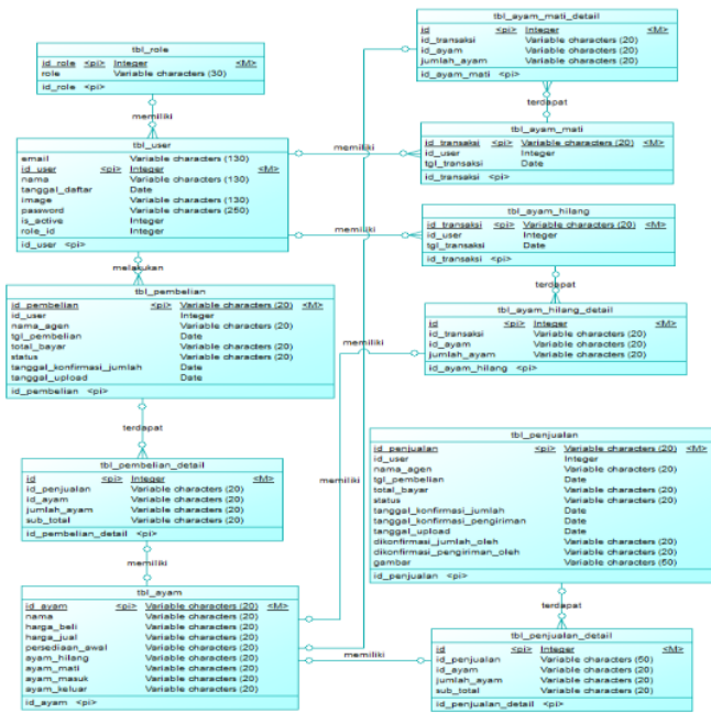
Gambar 3.3 CDM (Conceptual Data Model)
