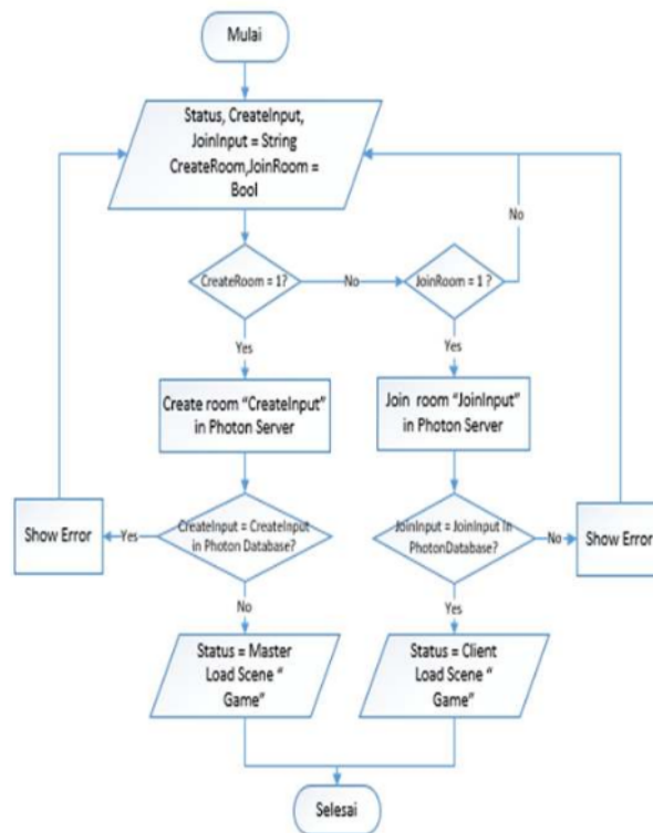
Gambar 4. 22 Flowchart create and join rooms
