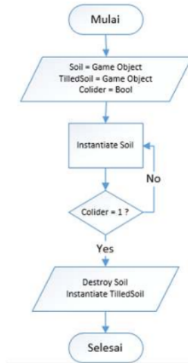
Gambar 4. 32 Flowchart soil tillage
