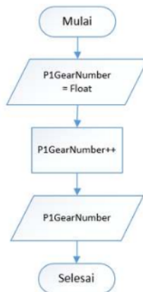
Gambar 4. 26 Flowchart input i
