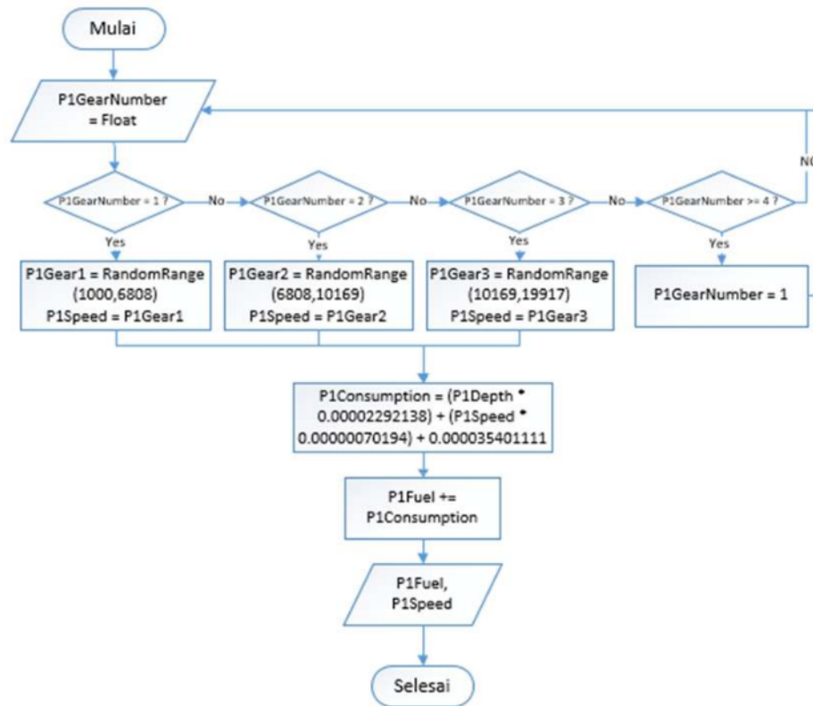
Gambar 4. 29 Flowchart add fuel
