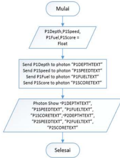
Gambar 4. 31 Flowchart send score to photon and show score
