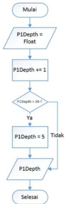
Gambar 4. 25 Flowchart input u
