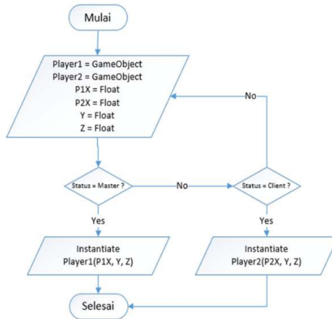
Gambar 4. 23 Flowchart spawn players
