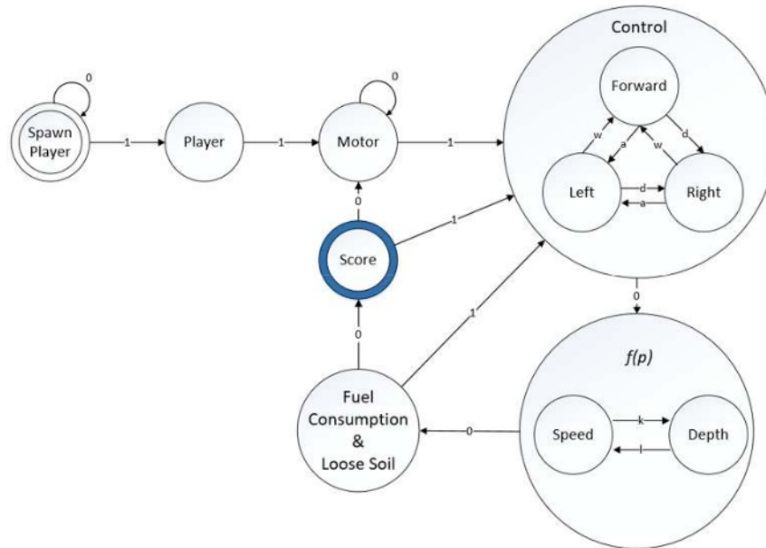
Gambar 4. 19 HFSM gameplay (Lee et al., 2022)
