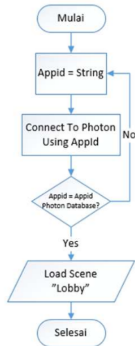
Gambar 4. 21 Flowchart connect to photon server
