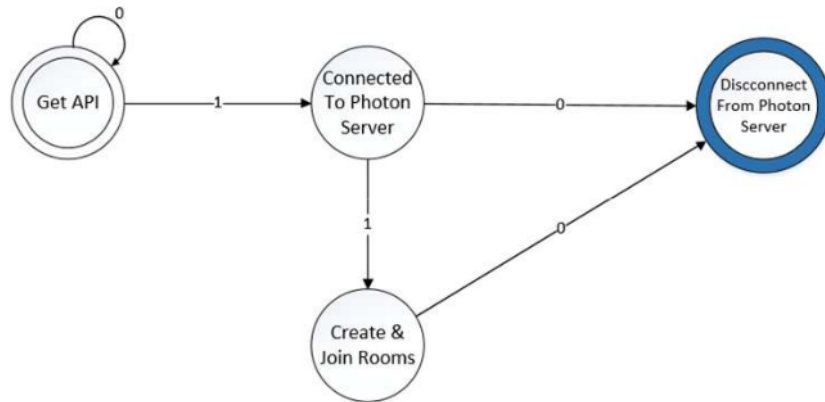
Gambar 4. 18 FSM multiplayer connection (Lee et al., 2022)
