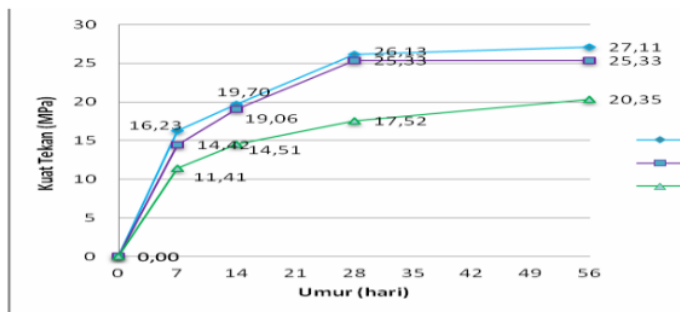
figure 4. bio-cement + molasses sample
