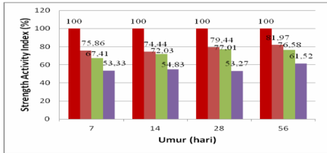
Figure 8. bio-cement plus molasses sample
