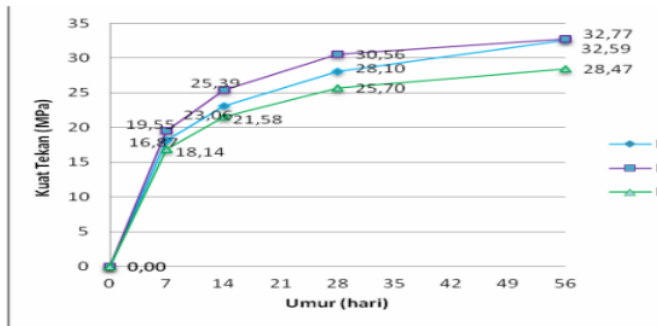
Figure 6. bio-cement "burn" plus molasses sample
