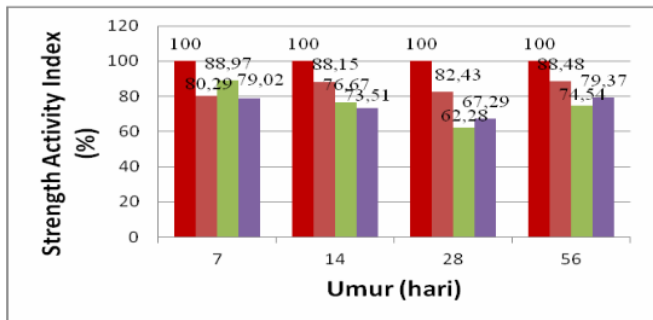
Figure 7. filtered bio-cement sample
