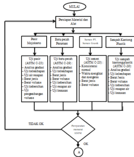
Gambar 1. Diagram alir
