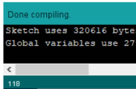
Gambar 6 compile done
