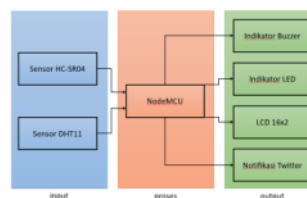
Gambar 2 Blok Diagram
