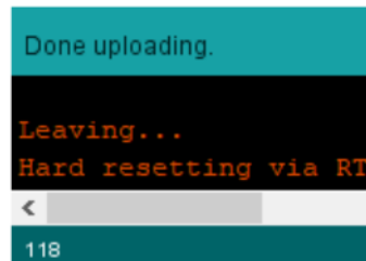
Gambar 7 done upload
