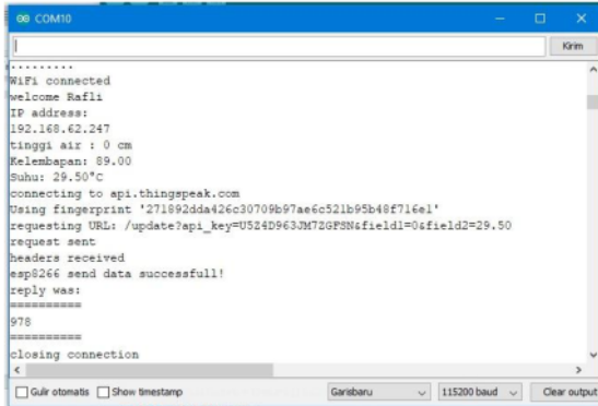
Gambar 8 Serial monitor
