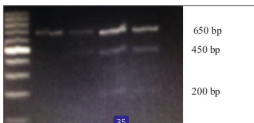
Figure 1. Gel electrophoresis of G gamma gene (-158 C>T) PCR-RFLP with XmnI restriction enzyme. Lane 1 (left side): DNA marker 100 bp, lane 2: 650 bp band from patient with XmnI (-/-) polymorphism, lane 3-5: 650bp, 450 bp and 200 bp bands from patients with XmnI (+/-) polymorphism.
