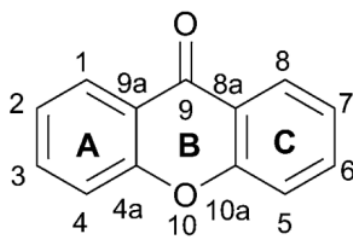
1 xanthone
