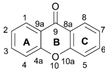
1 xanthone
