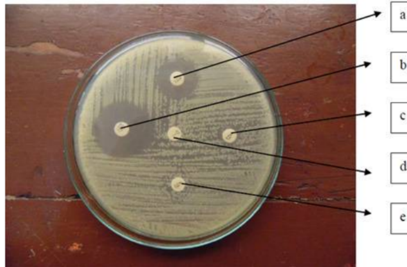
Fig. 1 : Antibiotic sensitivity test (a). Gentamycin antibiotic disk (b) Cefoperazone antibiotic disk (c) Erythromycin antibiotic disk (d) Oxacillin antibiotic disk (e) Penicillin antibiotic disk.
