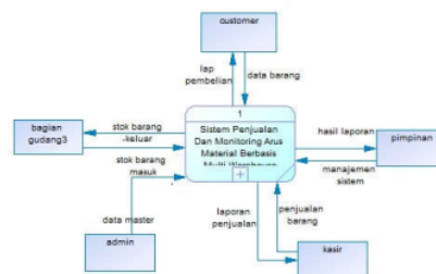
Gambar 2 Diagram Context
