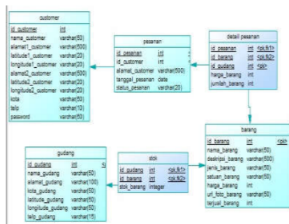
Gambar 11 PDM
