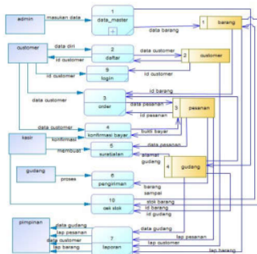
Gambar 8 DFD level 1
