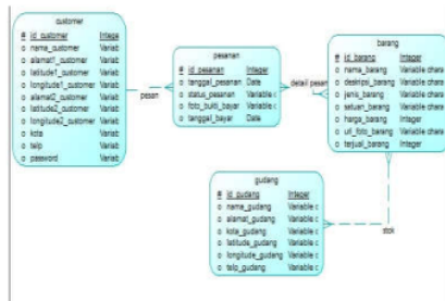
Gambar 10 CDM
