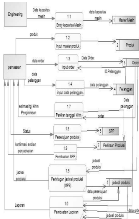
Figure 5 DFD Level 1
